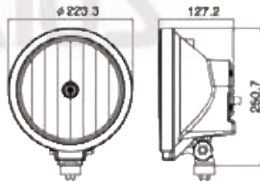
9" HID DRIVING LAMP
