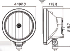
7" HID DRIVING LAMP
