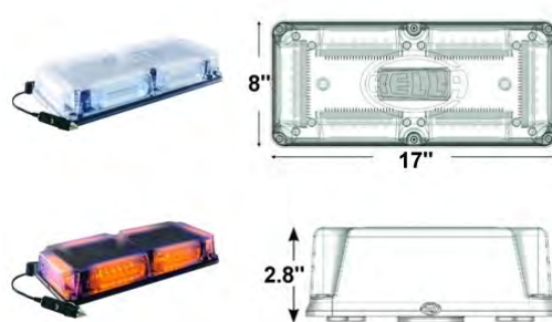
MLB 170 Mini Lightbar LED magnetic base 12V amber LEDs clear lens
