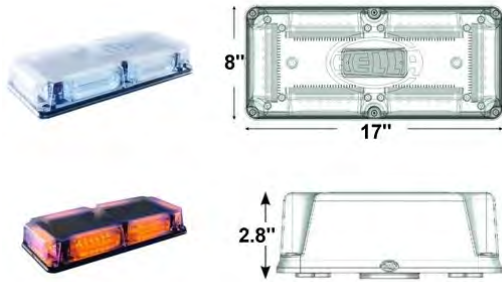
MLB 170 Mini Lightbar LED fixed base 12V amber LEDs clear lens
