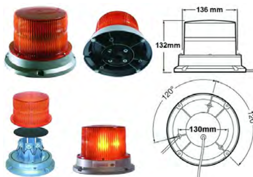
Model K-LED 450 Fixed multi-voltage amber LEDs amber lens
