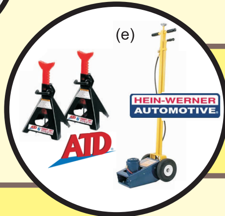
HWA-HW93733 - 20 ton axle jack ATD-7348 - Pair of Quick Lift Magic Lift Jack Stands – 12 Ton Capacity per Pair
