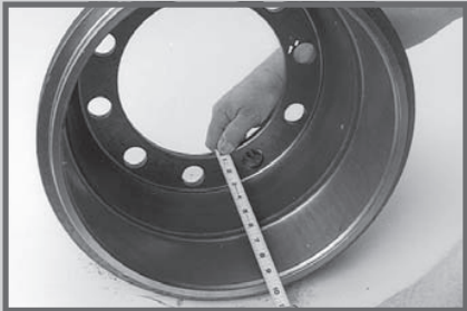
Figure 2 Overall depth of the drum
