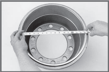
Figure 1 Inside diameter
